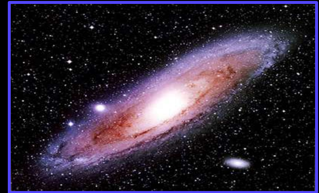
The Galactic Center Radiates Magnetic Energy.
