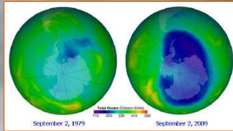
Ozone Hole over Antarctica 1979 - 2000 Comparison
