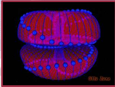
A Black Hole Vortex.
